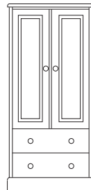
JJ8825 Childs Double Robe with Drawers H: 179cm/70.5" D: 56.5cm/22" W: 82.5cm/32.5"
